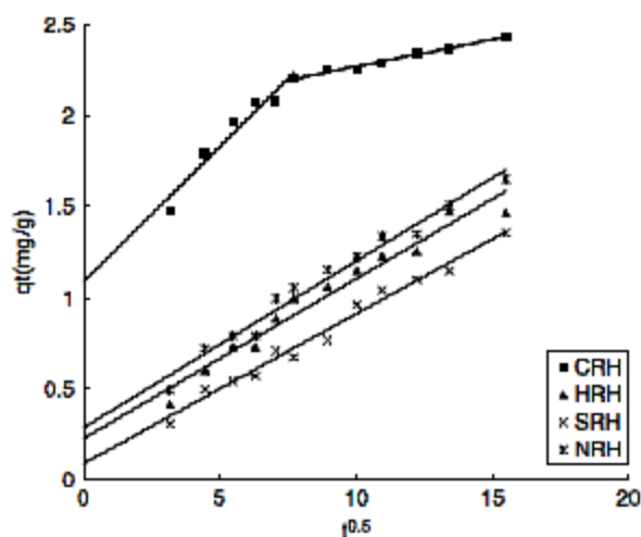
Fig. 5- Intraparticle-diffusion plot for the adsorption of MB onto various pretreated rice husks.
