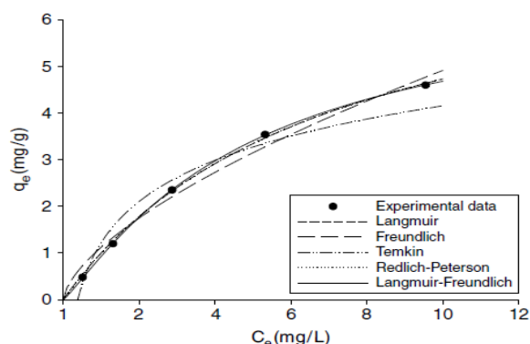
Fig. 8- Experimental points and comparison of the fitted curves from various adsorption isotherms for the adsorption of MB onto CRH.
