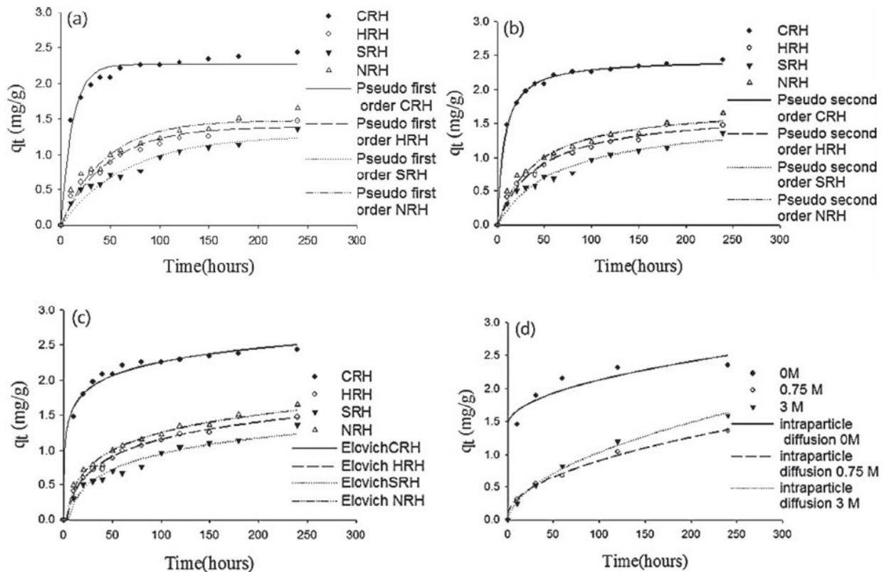
Fig 4- Comparison between the measured and modeled time profiles and comparison of kinetic models in predicting qt for the adsorption of MB onto various pretreated rice husks.
