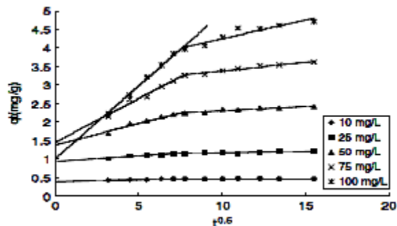
Fig.7- Intraparticle diffusion plot for the adsorption of MB onto CRH at different initial MB concentrations.
