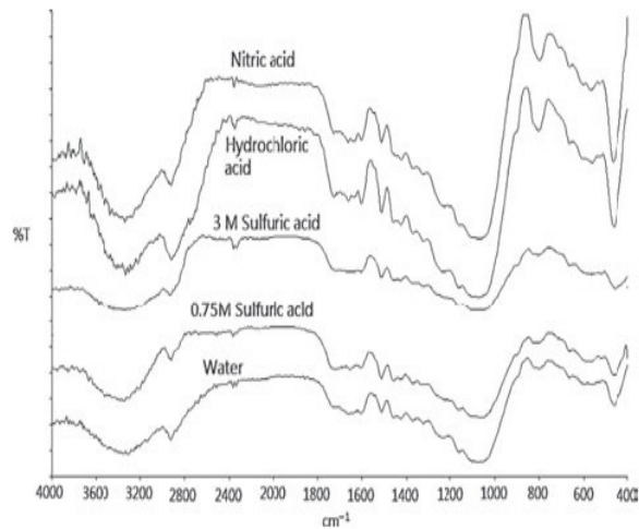
Fig.1- FTIR spectra for CRH, SRH, HRH, NRH.
