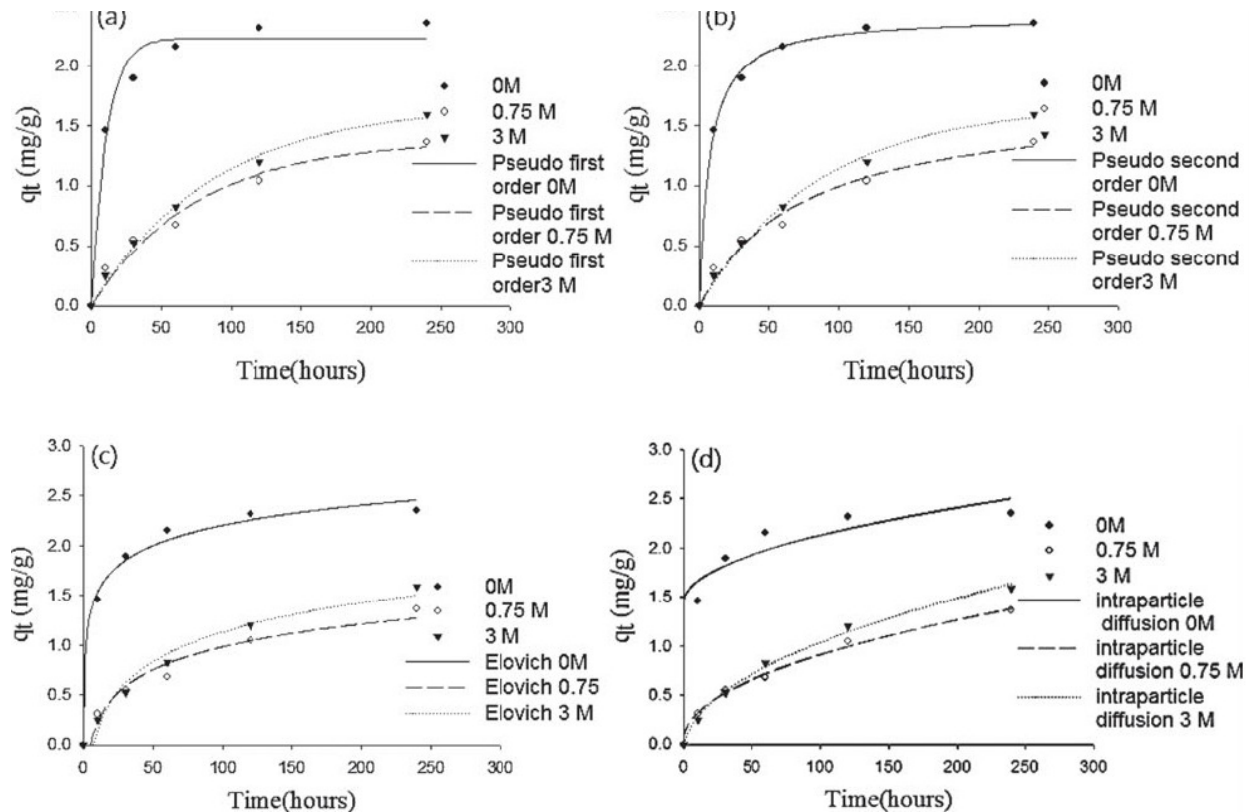
Fig. 2- Comparison between the measured and modeled time profiles and comparison of kinetic models in predicting q_t for the adsorption of MB onto CRHs modified by various acid concentrations.
