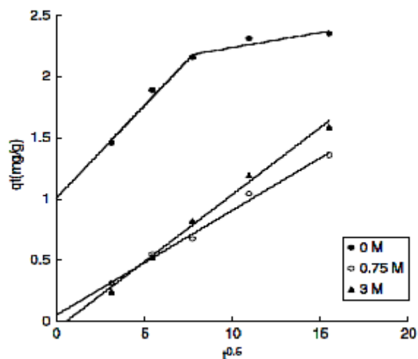
Fig 3- Intraparticle diffusion plot for the dsorption of MB onto CRHs modified by various acid concentrations.
